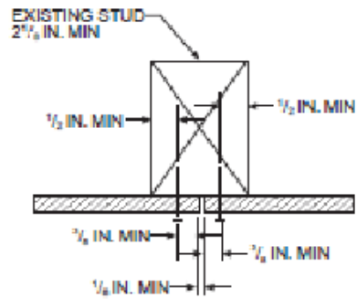
VERTICAL SPLICE AT SINGLE STUD
