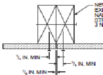
VERTICAL SPLICE AT DOUBLE STUD
